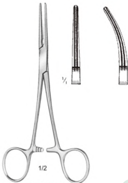
DE BAKY-RANKIN 120-0001 Straight 160mm (6.1/4") 120-0002 Curved 160mm (6.1/4")
